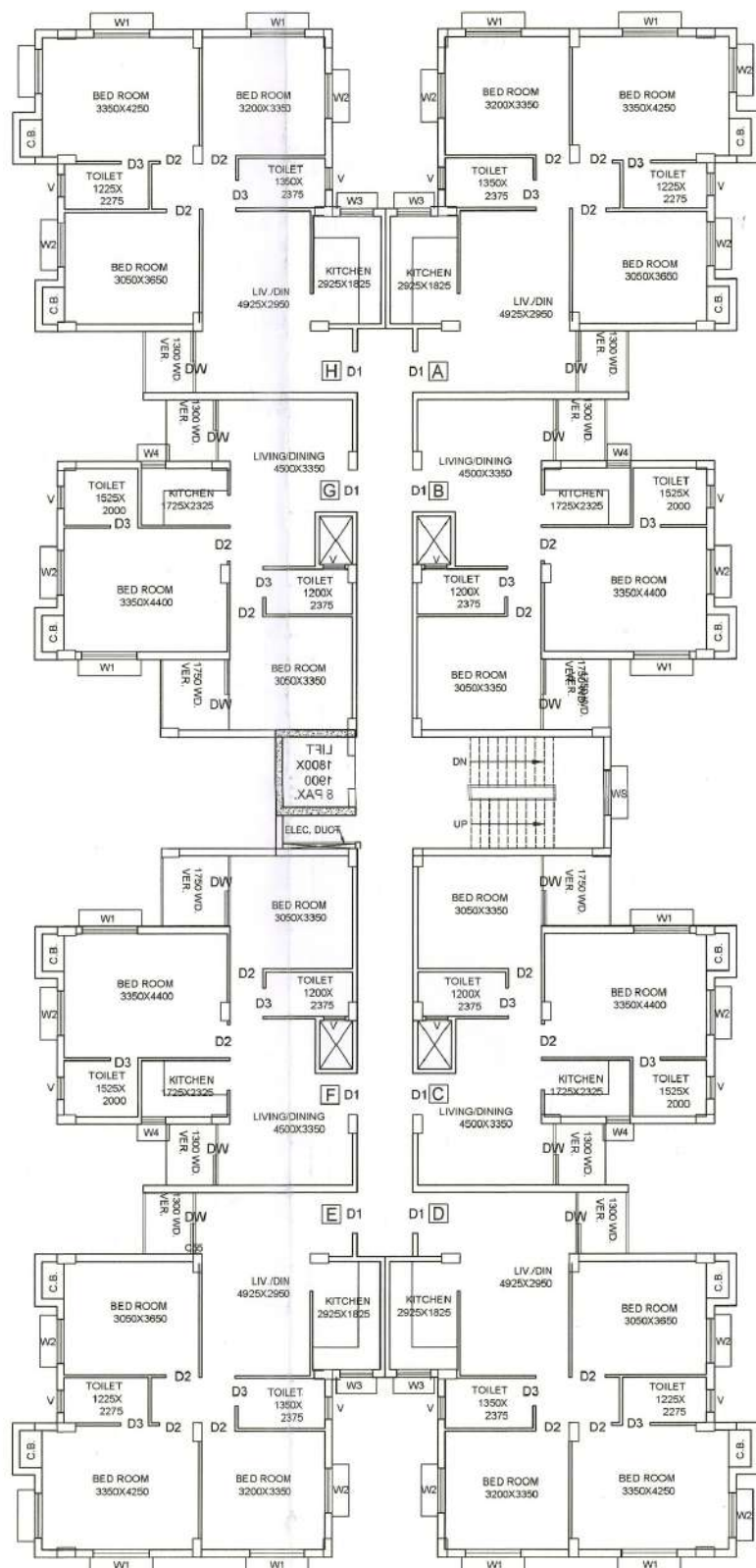
TYPICAL FLOOR PLAN (BLOCK-E)
